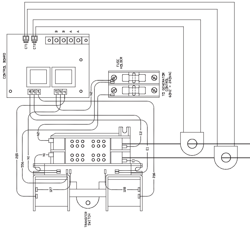
WIRE DIAGRAM
